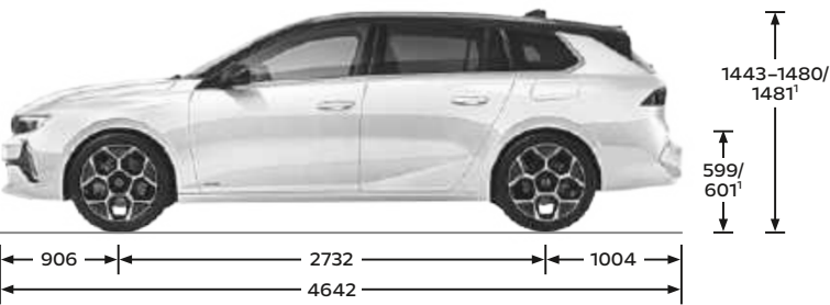
Astra Sports Tourer Tutte le misure in mm
