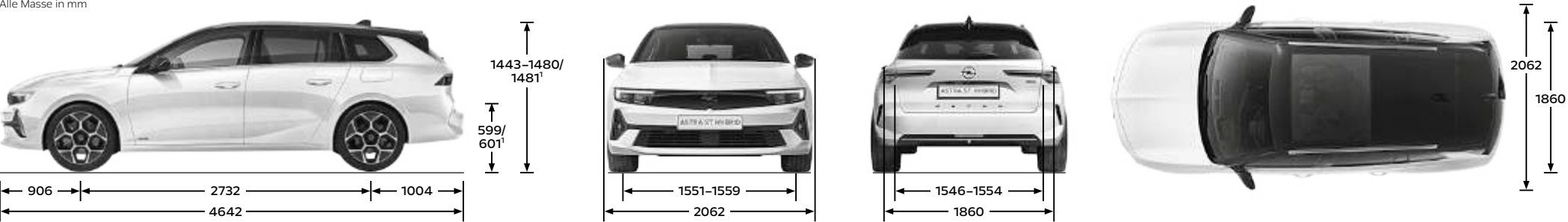
Astra Sports Tourer Alle Masse in mm
