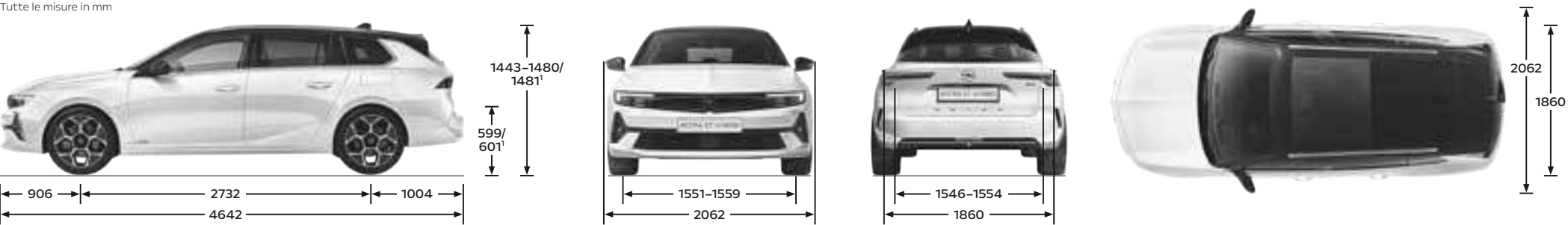
Astra Sports Tourer Tutte le misure in mm
